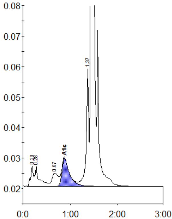
Peak table - ID: 10416690
